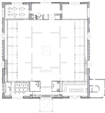
Grundriss / floor plan
