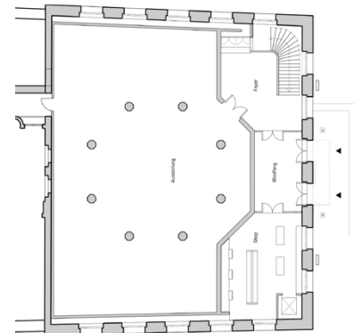
Grundriss EG / ground floor plan
